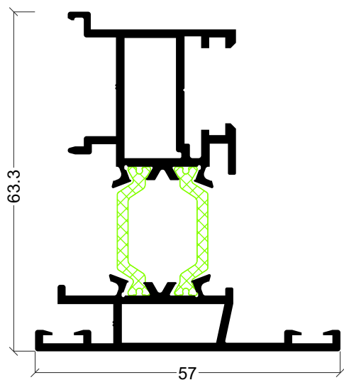
ARI-04 Inversor
