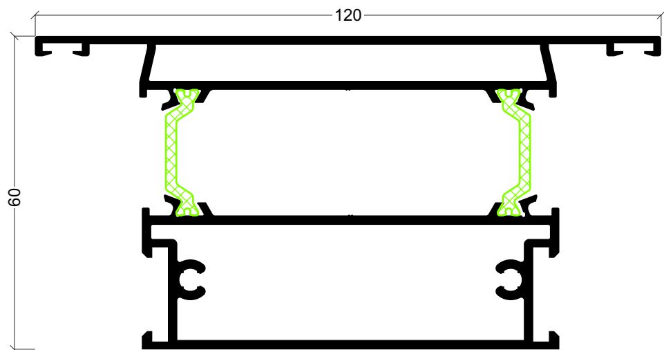
ARi-12 Travessa
