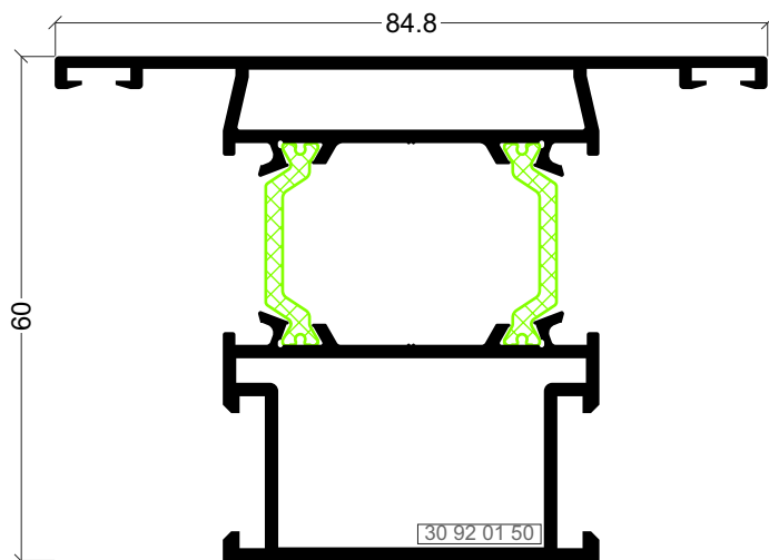
ARi-06 Travessa
